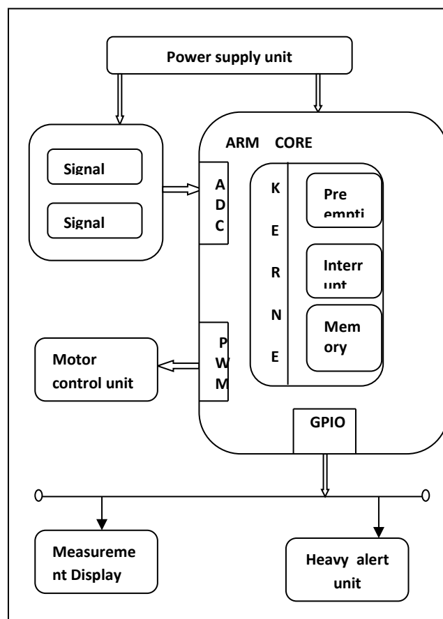
Fig 1: Block Diagram
