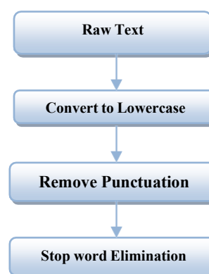
Fig 2 Data Preprocessing
